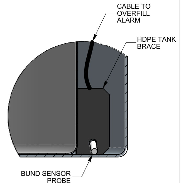
DETAIL C [BUND ALARM SENSOR] (1 : 6)
