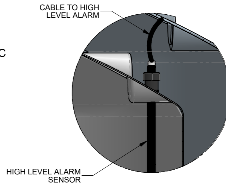
DETAIL B [HIGH LEVEL ALARM SENSOR] (1 : 7)
