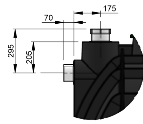
DETAIL A (INLET)
