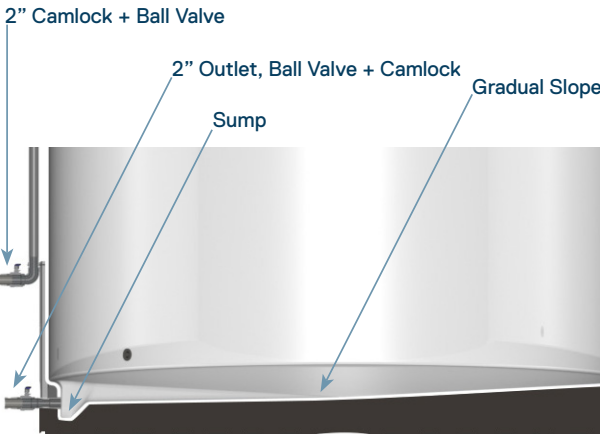
Self-Draining Tank Base
